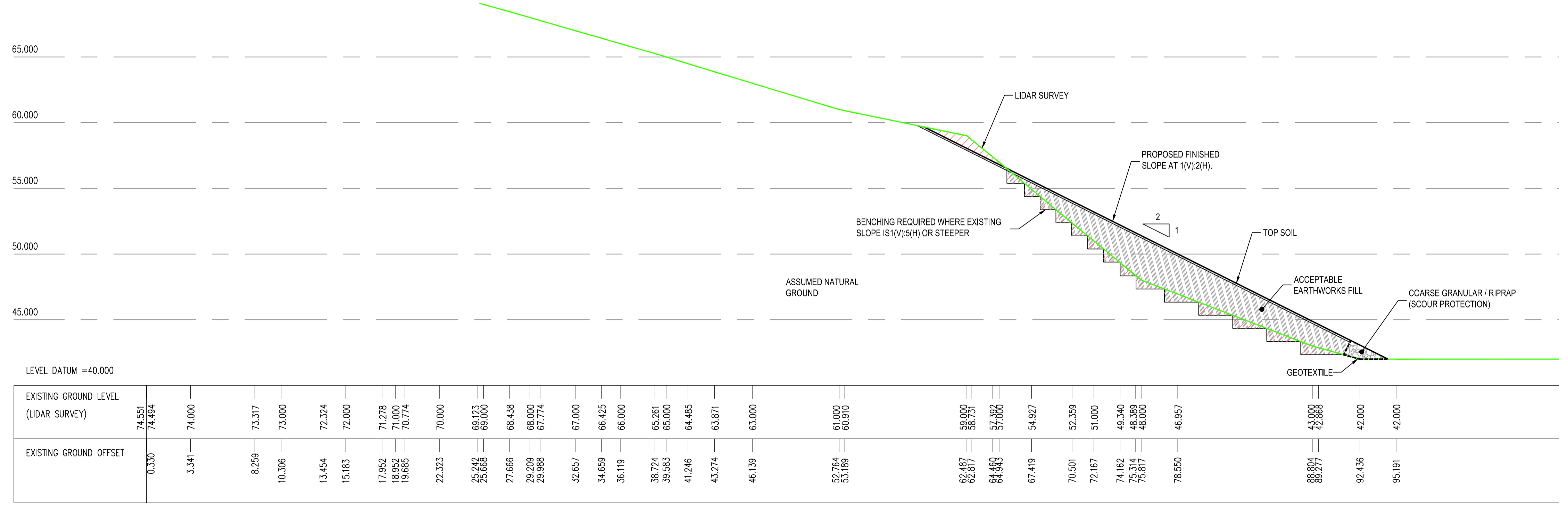
CROSS SECTION D-D
