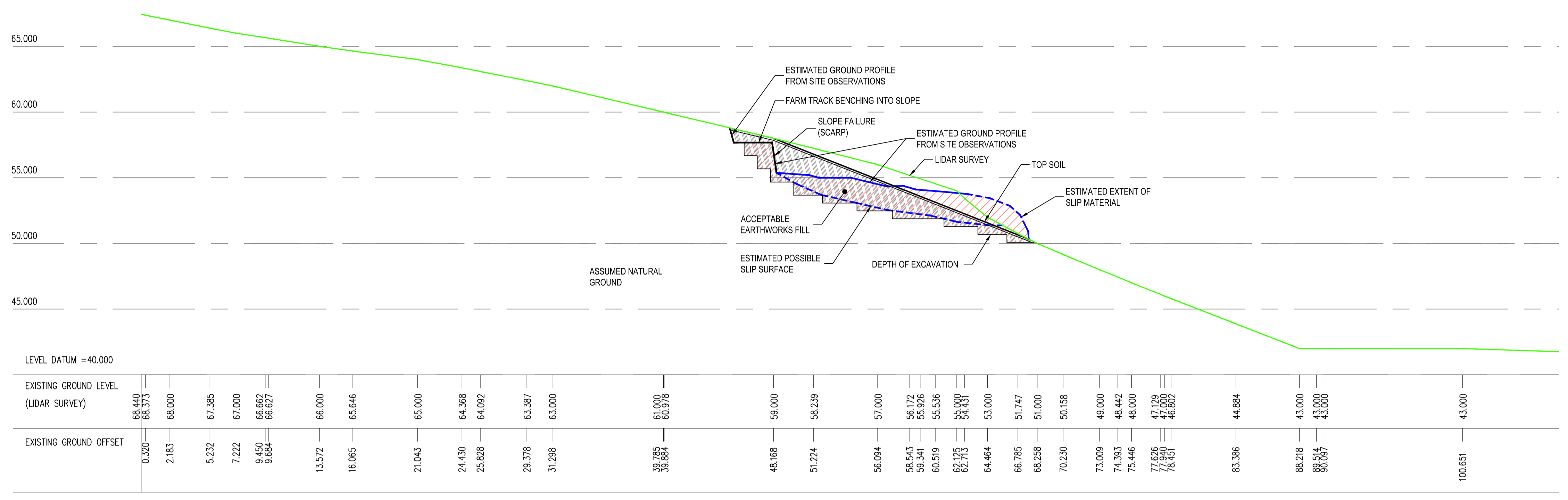
CROSS SECTION C-C
